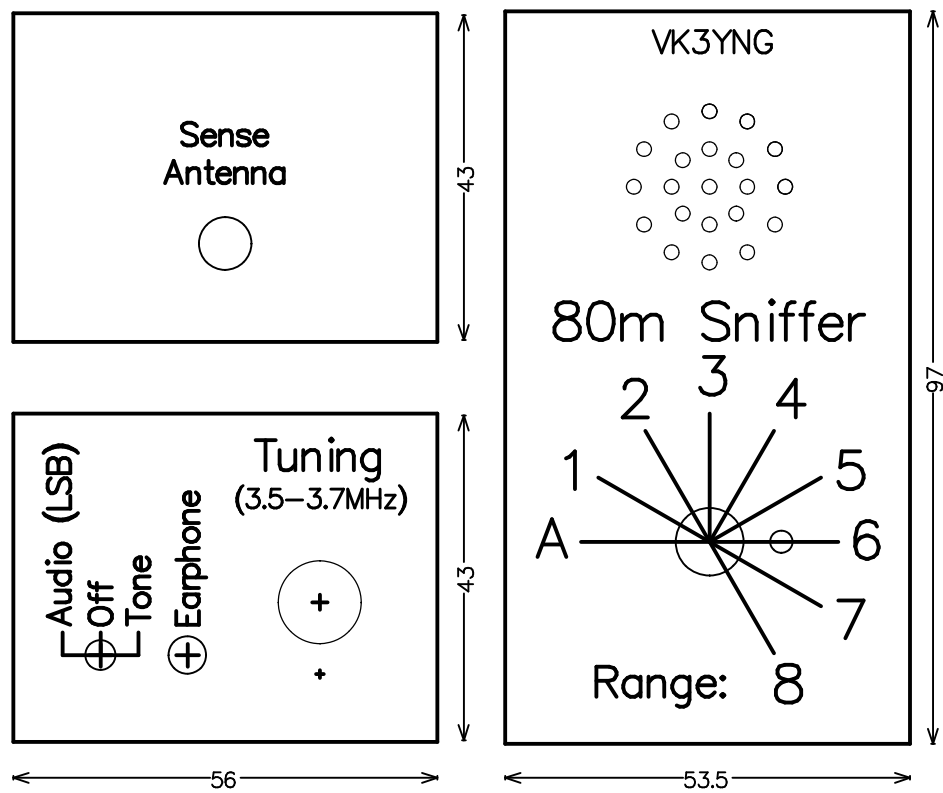
Figure 5 – Front and Side Panel Artwork
