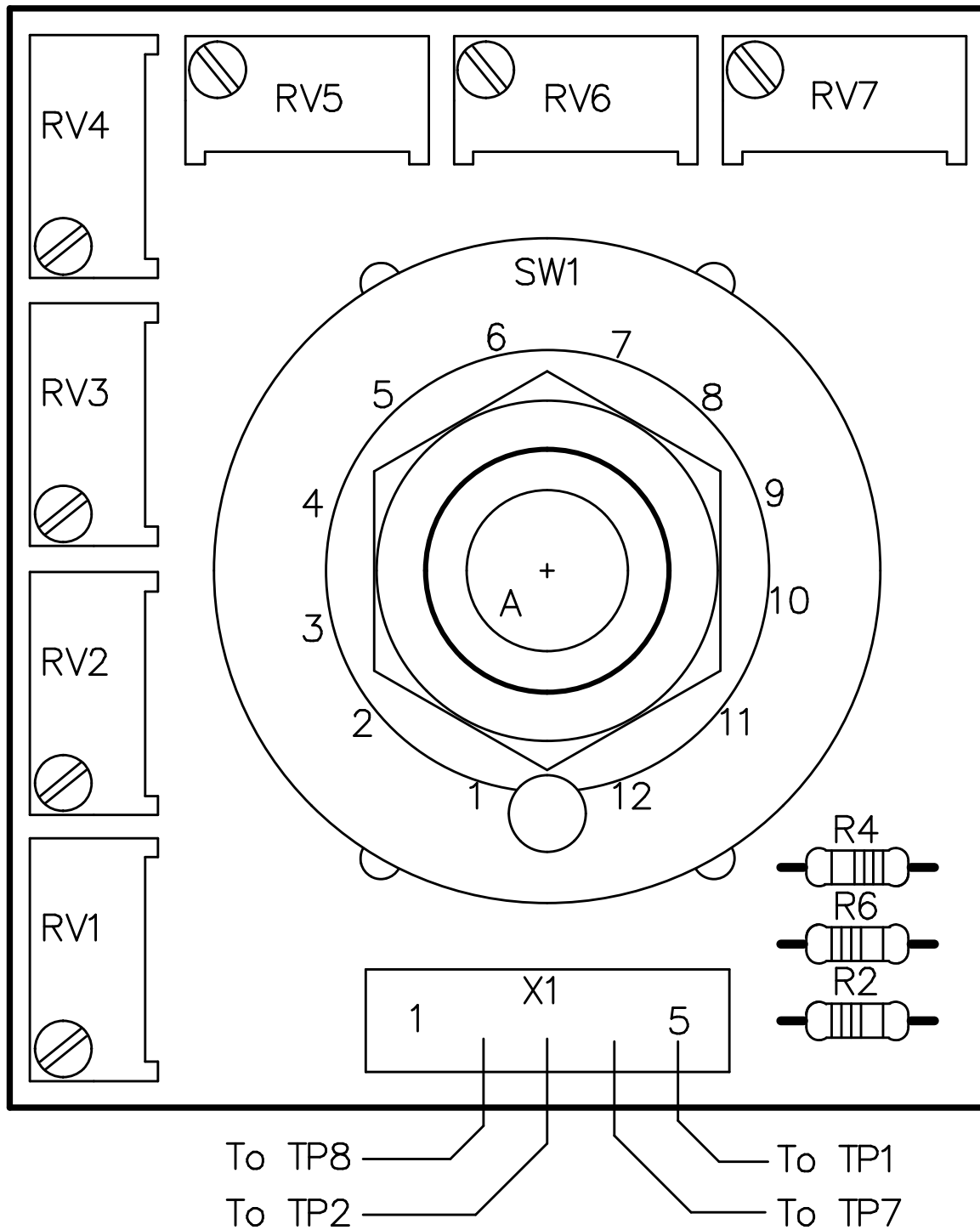
Figure 2 – PCB Top Assembly
