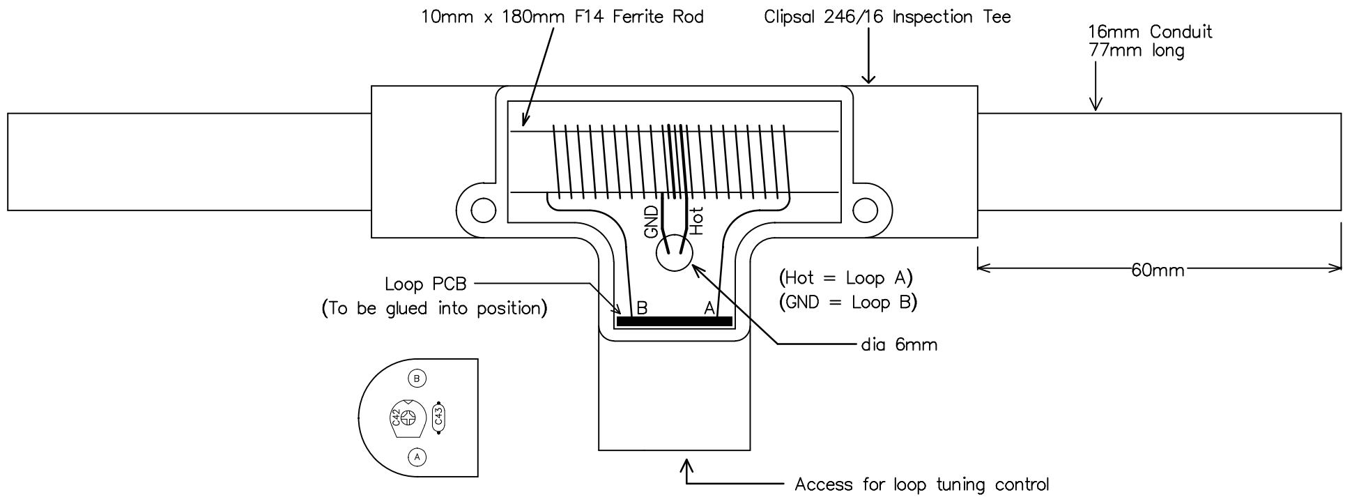
Figure 4 – Loopstick Assembly
