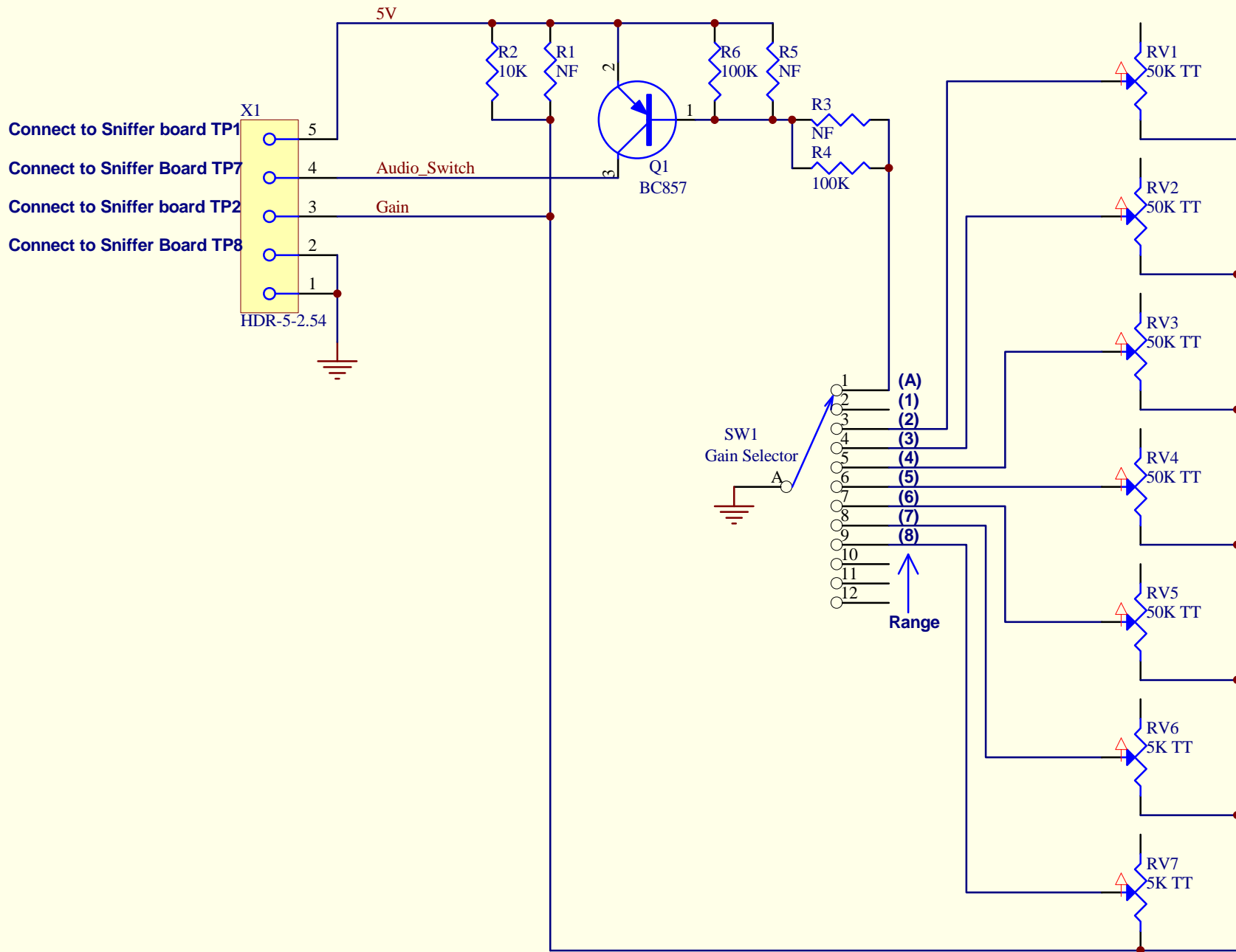
Figure 1 - 80M Sniffer Stepped Range Control
